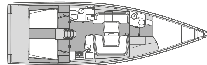
Option 2 - 4 cabins, 2 heads
